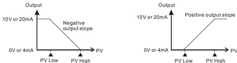
Figure 7: Proportional Output
